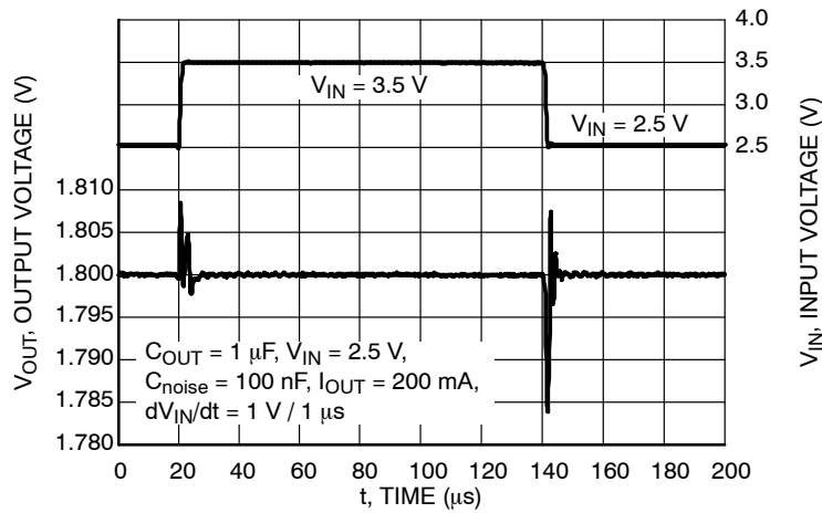
Figure 31. Line Transient Response, V_{\text{OUT}} = 1.8 \text{ V} , C_{\text{OUT}} = 1 \mu\text{F} , I_{\text{OUT}} = 200 \text{ mA}
