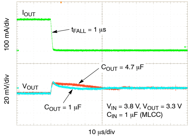
Figure 41. Load Transient Response - 250 \text{ mA to } 1 \text{ mA}
