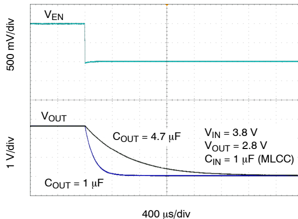
Figure 37. Enable Turn-off
