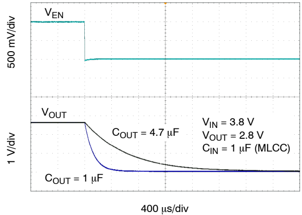
Figure 35. Enable Turn-off
