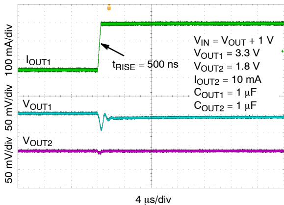
Figure 46. Load Transient Response - 3.3 V - Rising Edge, I_{OUT} = 50 \text{ mA} to 300 mA
