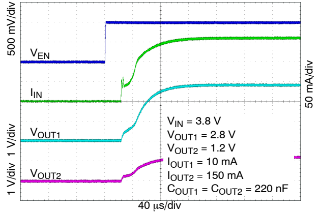
Figure 35. Enable Turn-on Response - VR1 = 10 mA, VR2 = 150 mA
