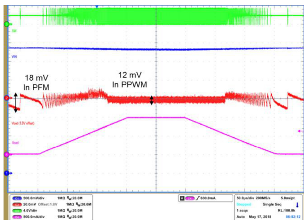
Figure 32. Ripple
