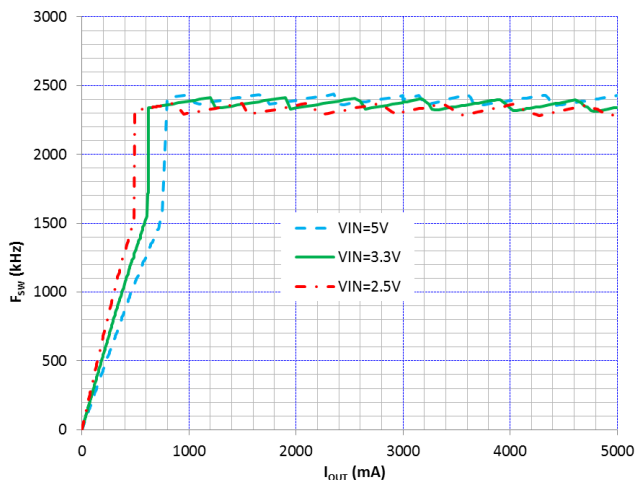
Figure 30. Switching Frequency vs I_{LOAD} and V_{IN} V_{OUT} = 1.10\text{ V}
