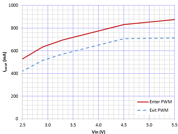
Figure 29. Switchover Point V_{OUT} = 1.4\text{ V}
