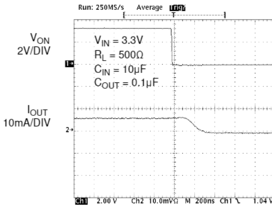
Figure 21. T_{OFF} Response
