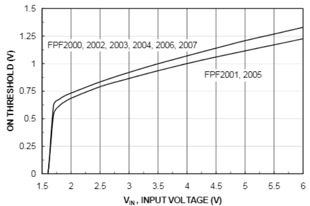
Figure 6. V_{HI} vs. V_{IN}
