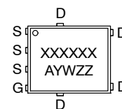
DFN5 (SO-8FL)
