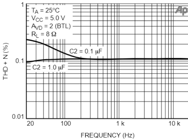
Figure 2. THD + N vs. Frequency (P L = 500 mW)
