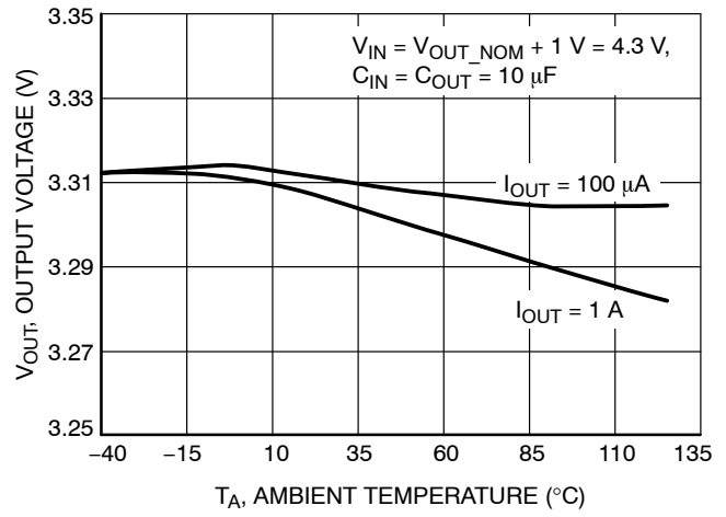
Figure 14. Output Voltage vs. Temperature ( V_{out} = 3.3\text{ V} )
