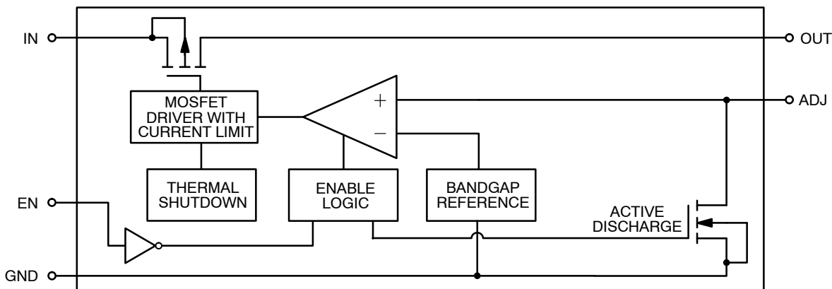
Figure 9. NCP691 Block Diagram (Adjustable Version)
