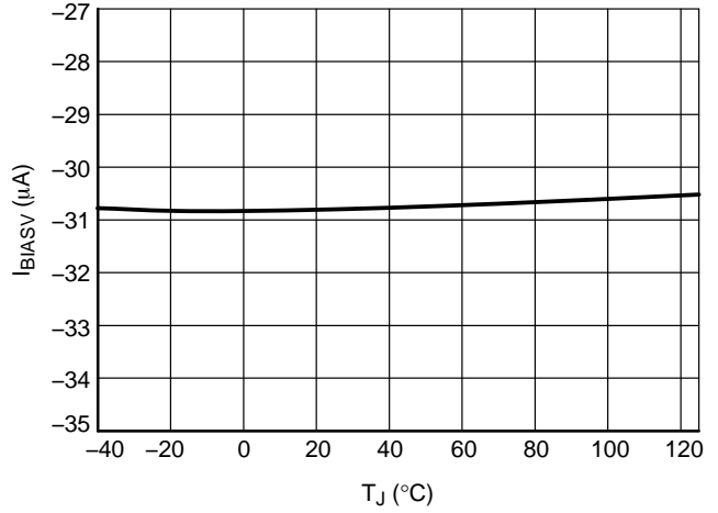
Figure 9. I BIASV at V CC = 15 V, V SNS > V SNSBIASLTH , V ECDETH < 10% V CC
