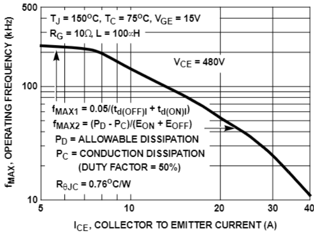
FIGURE 13. OPERATING FREQUENCY vs COLLECTOR TO EMITTER CURRENT
