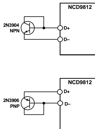
Figure 11. Remote Diode Connections Example
