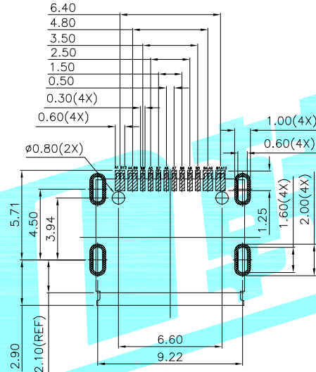
RECOMMENDED PCB LAYOUT(TOP VIEW) THICKNESS 0.8MM;DEFAULT TOLERANCE:±0.05
