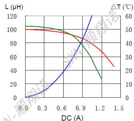
SMRH8D38-330N
