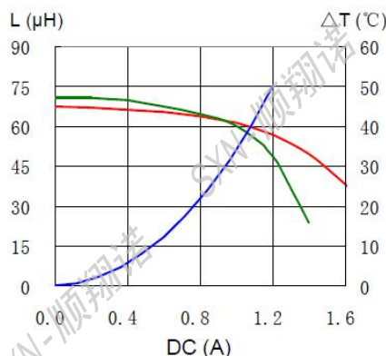
SMRH8D38-220N
