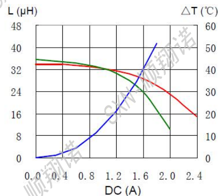
SMRH8D38-330N
