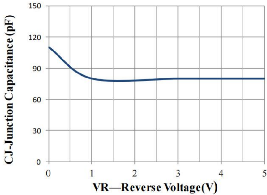
Junction Capacitance vs. Reverse Voltage
