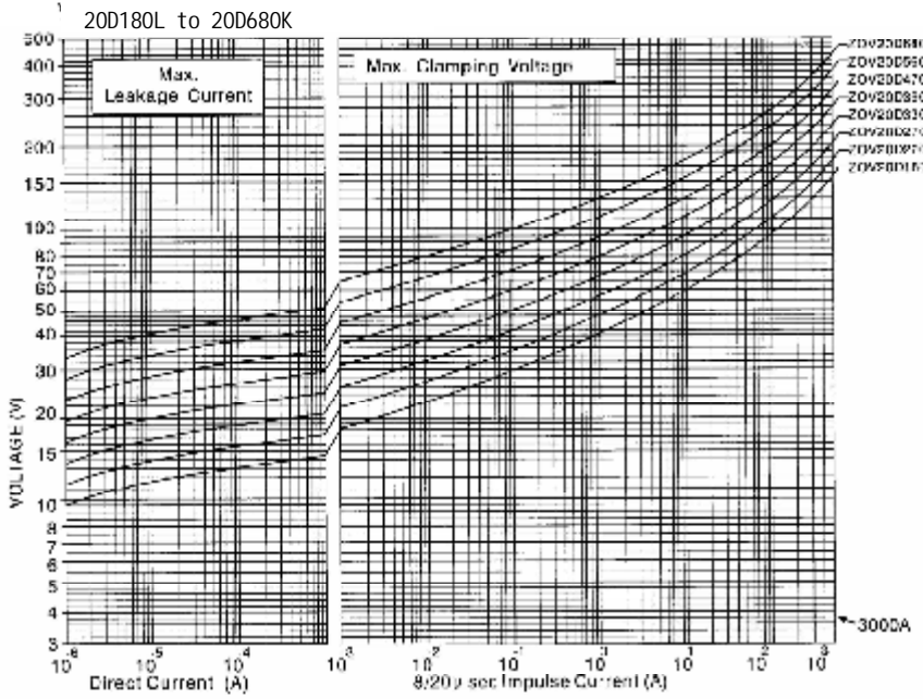
V-I Curve
