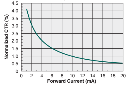
Single Transistor Typical Normalized CTR vs. I_F ( V_{CE}=0.5\text{V} )
