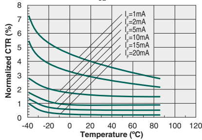
Single Transistor Typical Normalized CTR vs. Temperature ( V_{CE}=0.5\text{V} )
