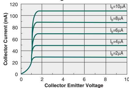
Typical Transfer Characteristics Darlington Transistor
