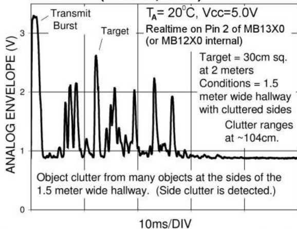
Analog Envelope Output (Clutter, 5.0V)
