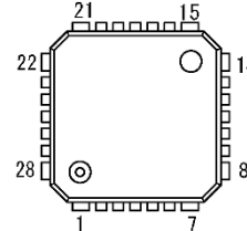
HQFN0808-28 Pin Configuration
