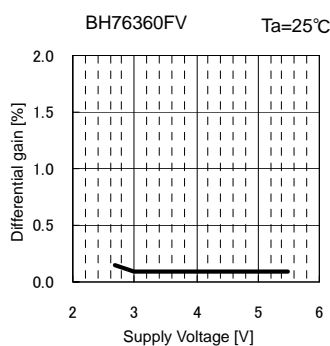
Fig.47 DG vs. Supply Voltage
