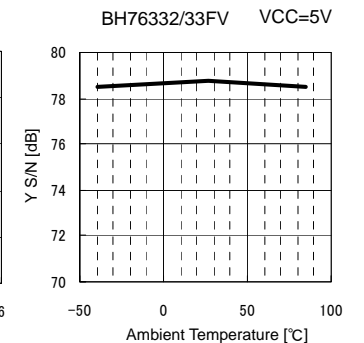
Fig.96 SN_Y vs. Ambient Temperature
