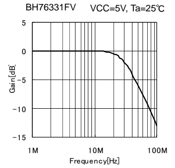
Fig.40 Frequency Response
