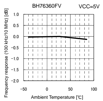
Fig.36 G f vs. Ambient Temperature
