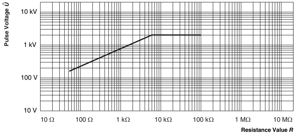
Pulse load rating in accordance with IEC 60115-1, 4.27; 1.2 \mu s/50 \mu s; 5 pulses at 12 s intervals; for permissible resistance change 0.5 %
