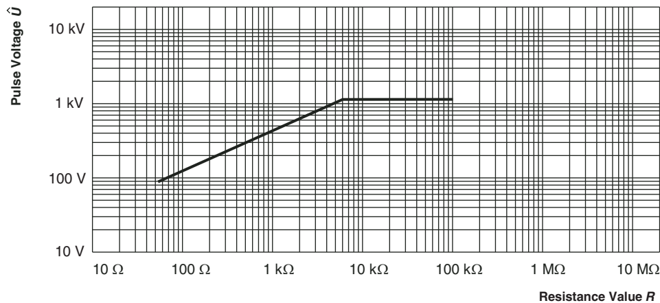
Pulse load rating in accordance with IEC 60115-1, 4.27; 10 \mu s/700 \mu s; 10 pulses at 1 min intervals; for permissible resistance change 0.5 %
