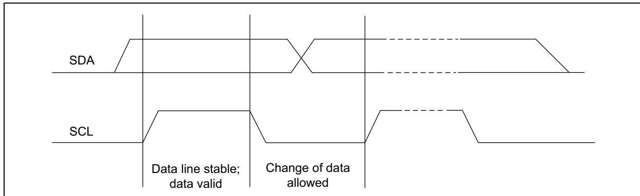
FIGURE 6-1: Bit Transfer.
