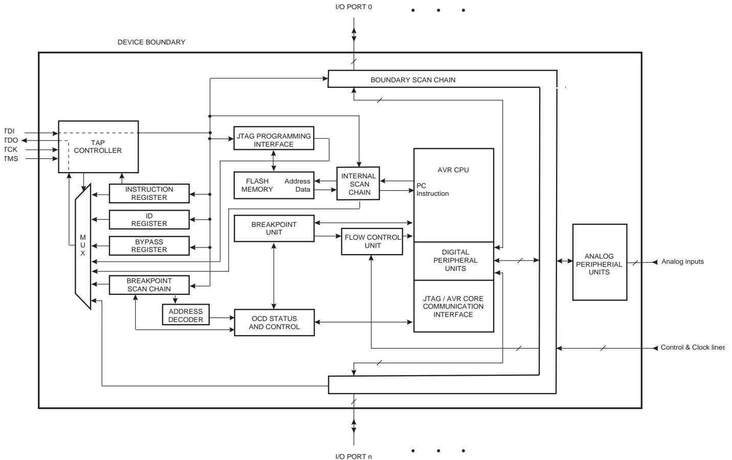
Figure 24-1. Block diagram
