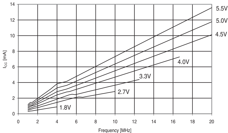
Figure 30-198. ATmega644A: Active supply current vs. frequency (1 - 20MHz)
