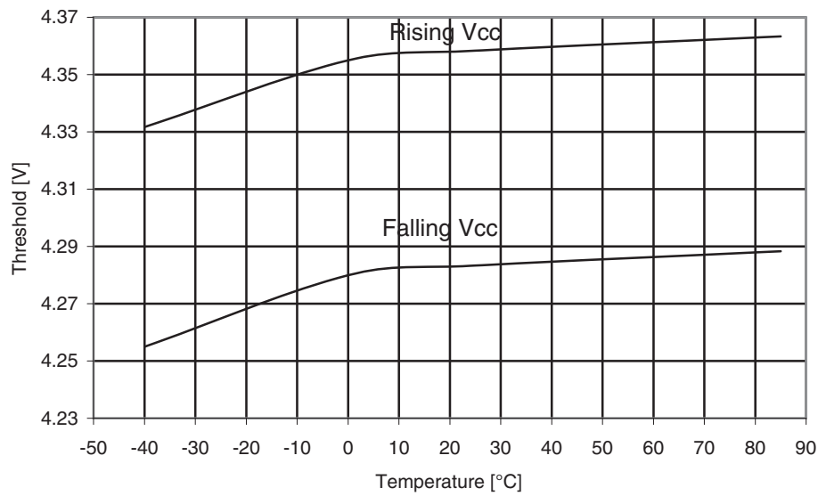
Figure 30-326. ATmega1284: BOD threshold vs. temperature ( V_{BOT} = 4.3V )
