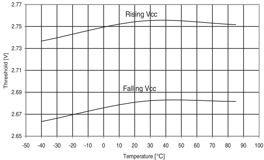
Figure 30-228. ATmega644A: BOD threshold vs. temperature ( V_{BOT} = 2.7V )
