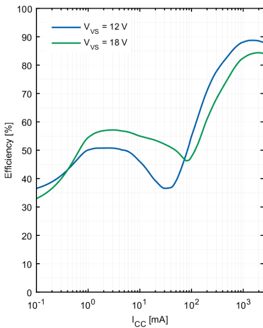
Efficiency FREQ: 2.2 MHz; T_j = 25^\circ\text{C}
