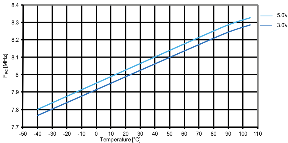
Figure 31-33. ATmega164PA: Calibrated 8MHz RC oscillator vs. temperature
