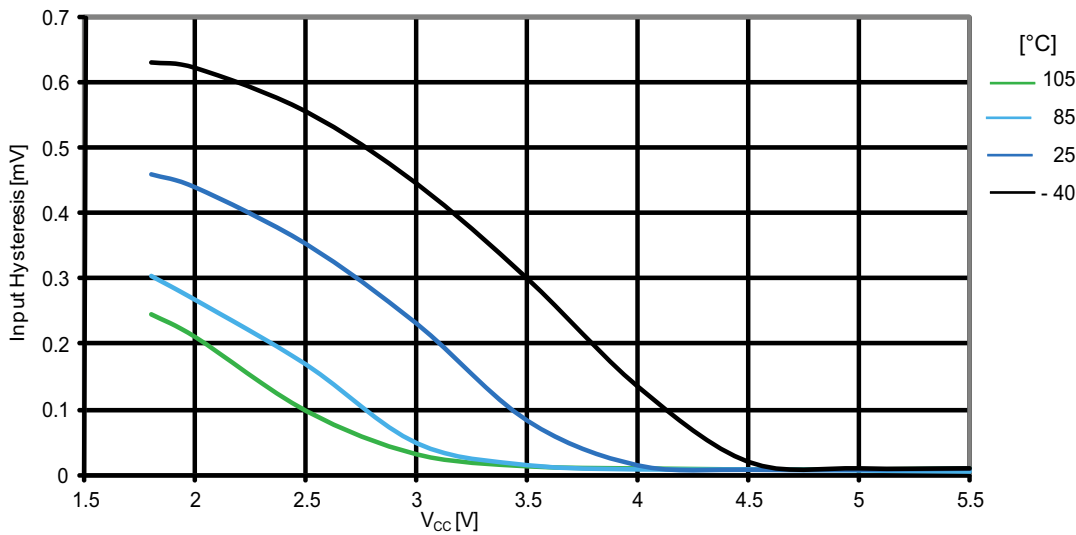
Figure 31-24. ATmega164PA: Reset pin input hysteresis vs. V_{CC}
