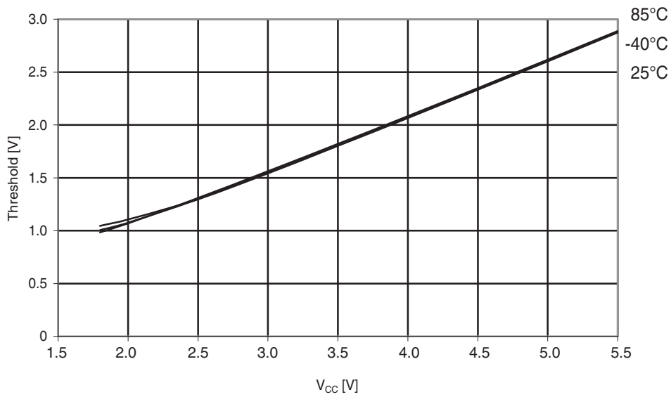
Figure 30-123. ATmega324A: I/O pin input threshold vs. V_{CC} ( V_{IH} , I/O pin read as '1')
