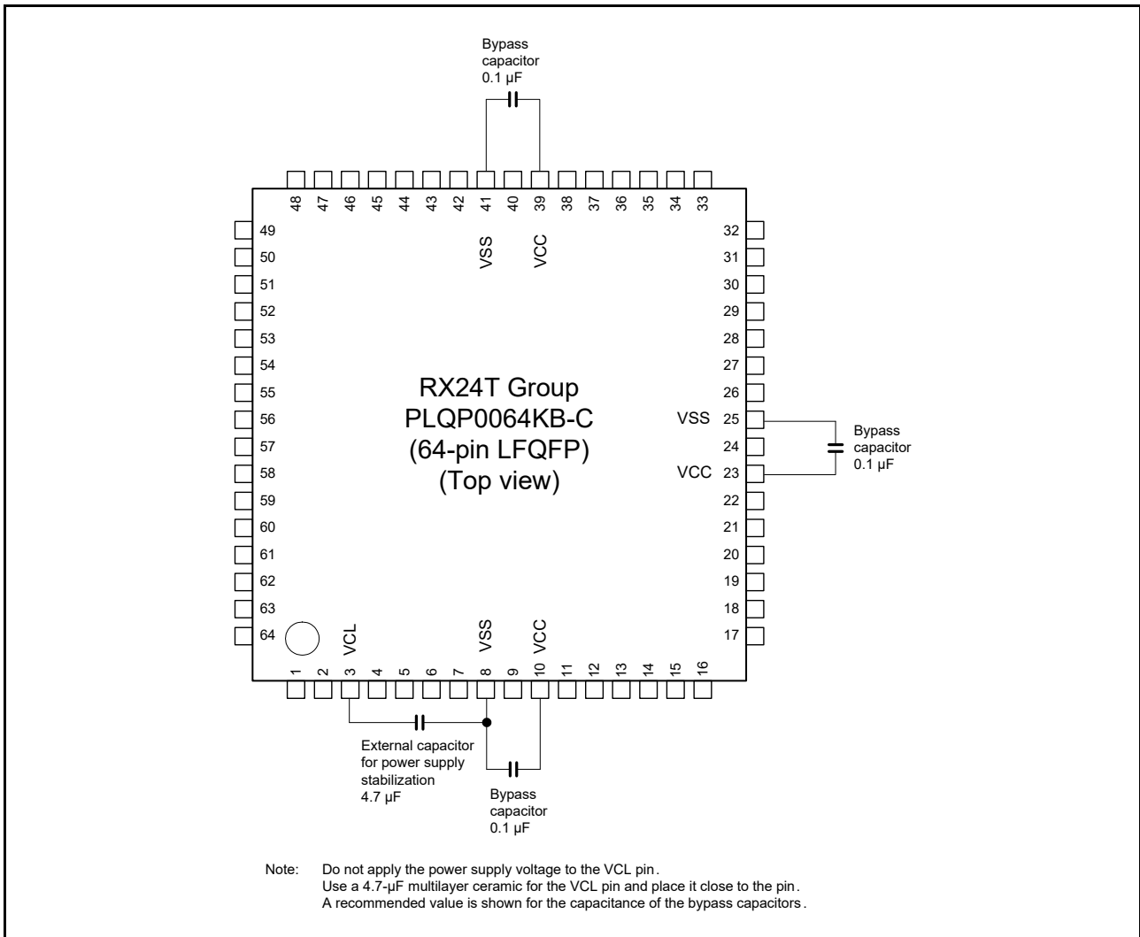
Figure 5.63 Connecting Capacitors (64 Pins)
