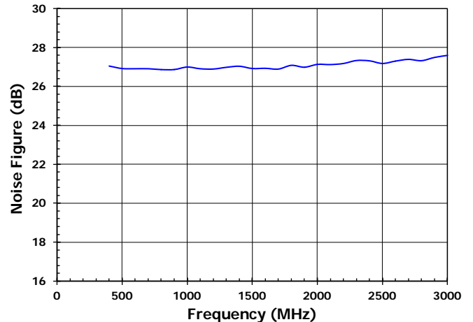
Figure 18. Noise Figure with DSA1=22 dB
