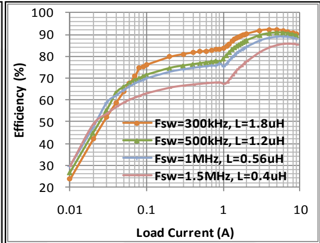
Figure 7. FAN23SV06 Efficiency vs. Load Current with V_{IN}=12\text{ V} and V_{OUT}=1.2\text{ V}
