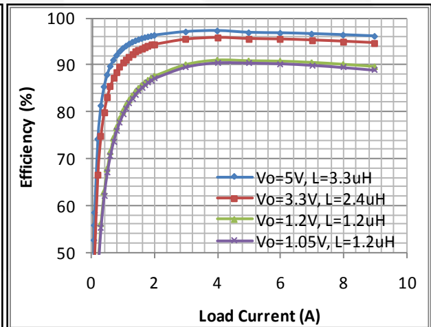
Figure 9. FAN23SV06P Efficiency vs. Load Current V_{IN}=12\text{ V} and f_{SW}=500\text{ kHz}
