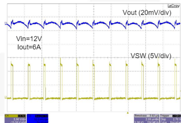
Figure 22. Static Output Ripple at Full Load
