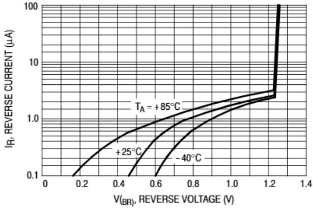
Figure 2. Reverse Characteristics
