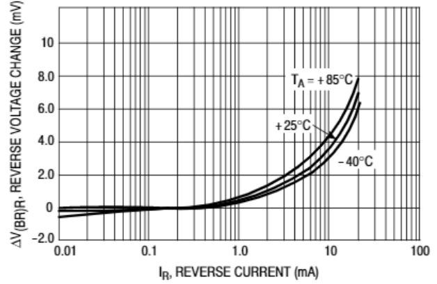
Figure 3. Reverse Characteristics
