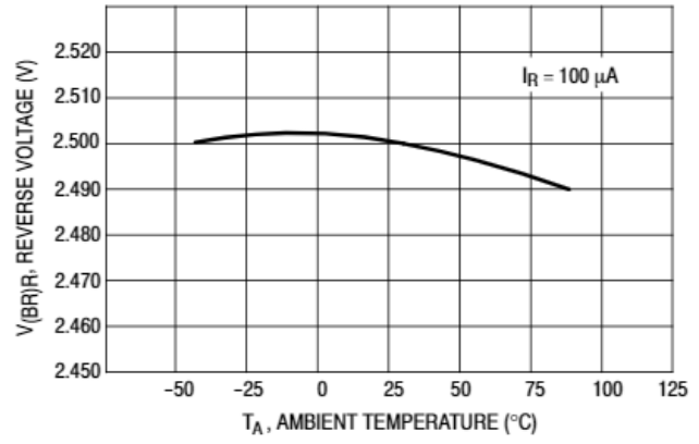
Figure 11. Temperature Drift
