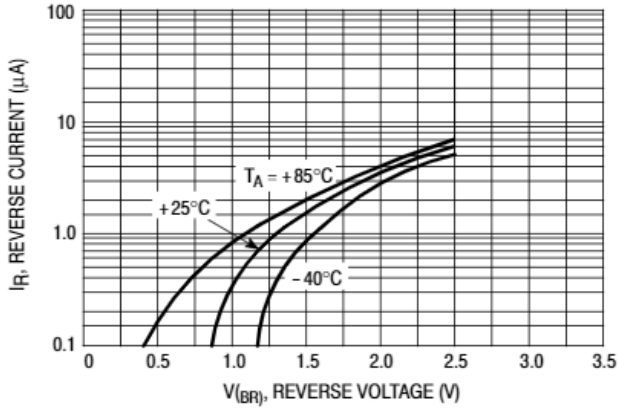
Figure 8. Reverse Characteristics
