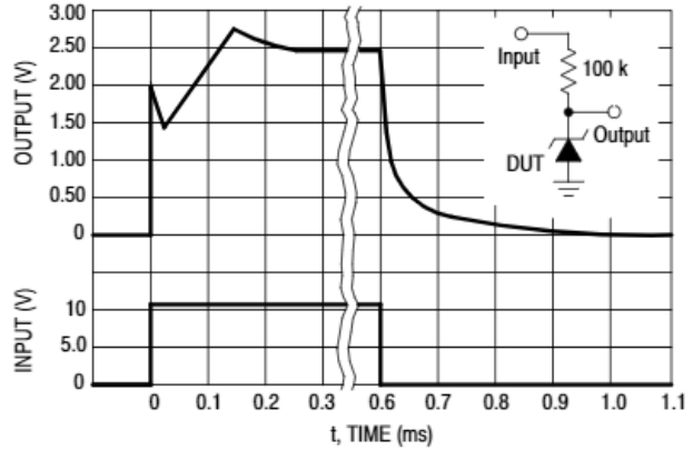
Figure 13. Response Time
