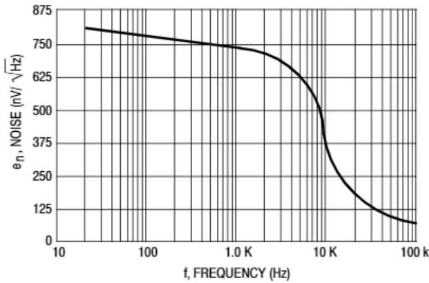
Figure 6. Noise Voltage
