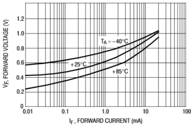
Figure 4. Forward Characteristics
