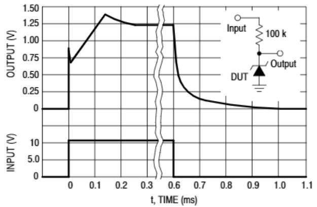
Figure 7. Response Time
