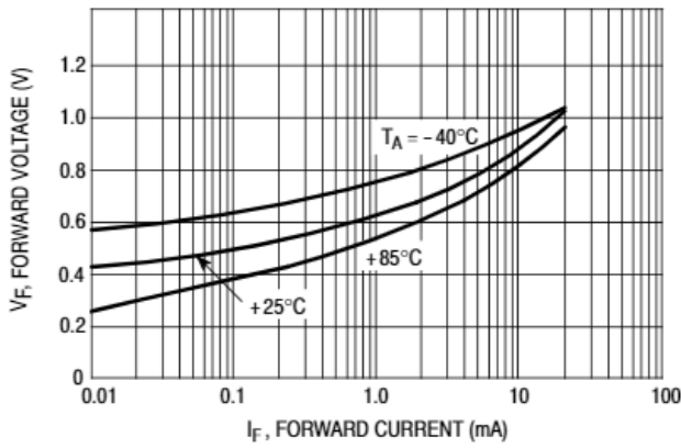
Figure 10. Forward Characteristics
