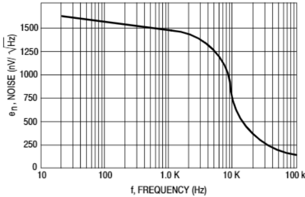
Figure 12. Noise Voltage
