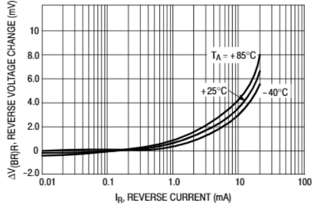
Figure 9. Reverse Characteristics
