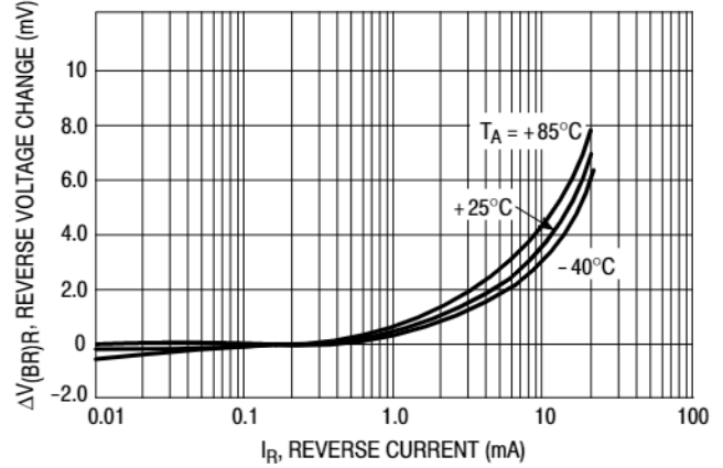
Figure 3. Reverse Characteristics
