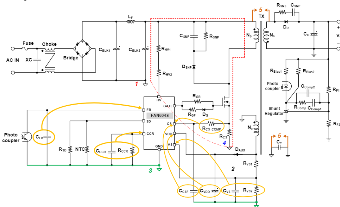
Figure 39 Recommended Layout for FAN604S
