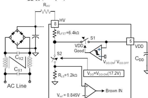
Figure 31 HV Startup Circuit
