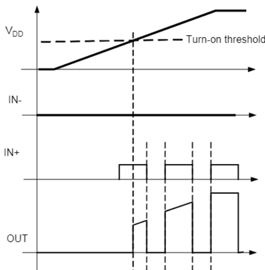
Figure 51. Non-Inverting Driver
