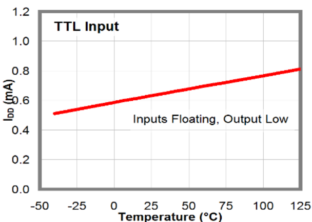
Figure 17. I_{DD} (Static) vs. Temperature (14)
