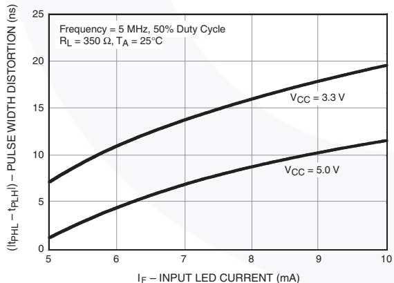
Figure 13. Pulse Width Distortion vs. Input LED Current ( I_F )
