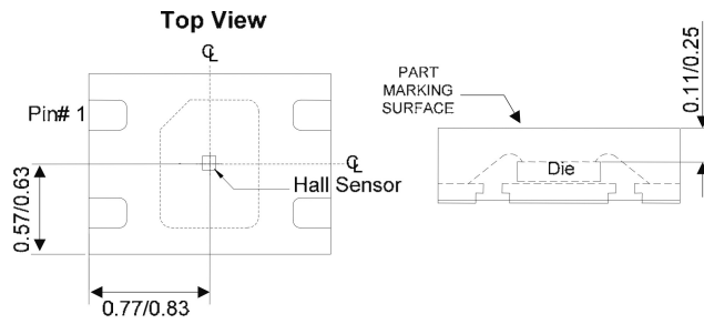
Sensor Location
