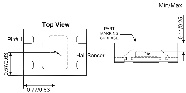
Sensor Location
