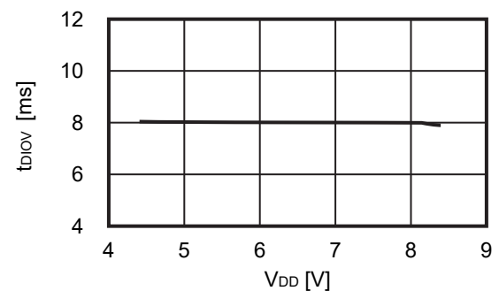
2.8 t_{DIOV} - V_{DD}
