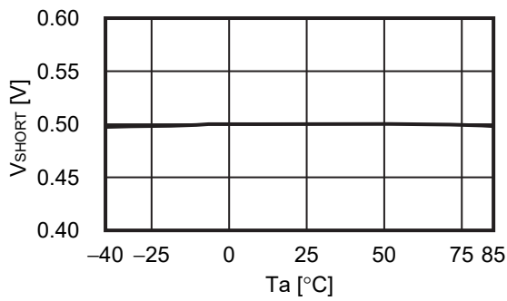
2.13 V_{SHORT} - T_a
