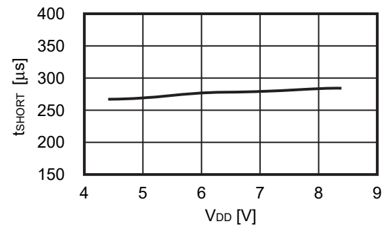
2.14 t_{SHORT} - V_{DD}
