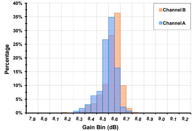
Gain Distribution ( F_{RF} = 915 MHz, LC mode, N = 1598)
