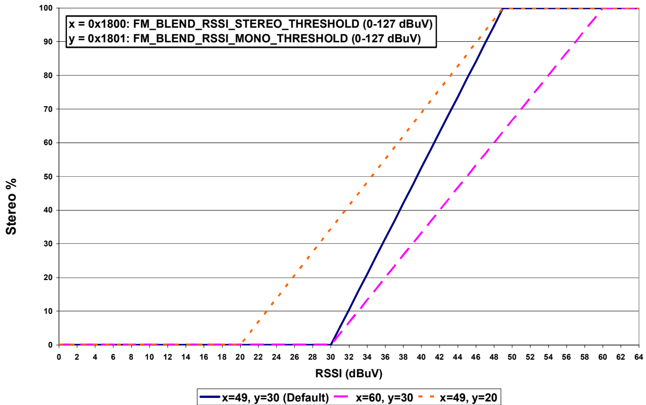
Figure 4. RSSI Blend
