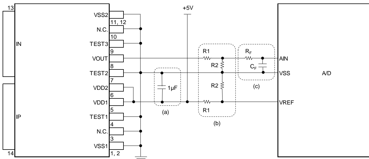
Figure 6. Recommended external circuits of AK310H
