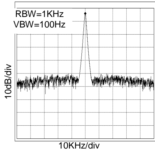
Figure 18. 17.7MHz Spectrum (At V_{DD}=3.3V and C_L=15pF )
