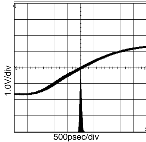
Figure 20. 14.3MHz Period-Jitter (At V_{DD}=3.3V and C_L=15pF )
