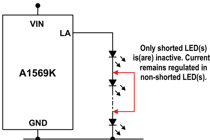
Figure 8: Shorted LED(s)
