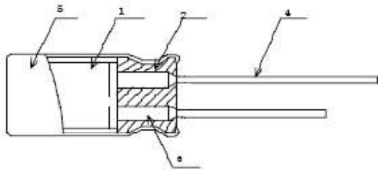
Fig. 1 Cross-section view
